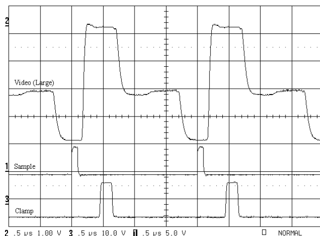
Figure 5 Two columns combined (binned) on to the floating diffusion
