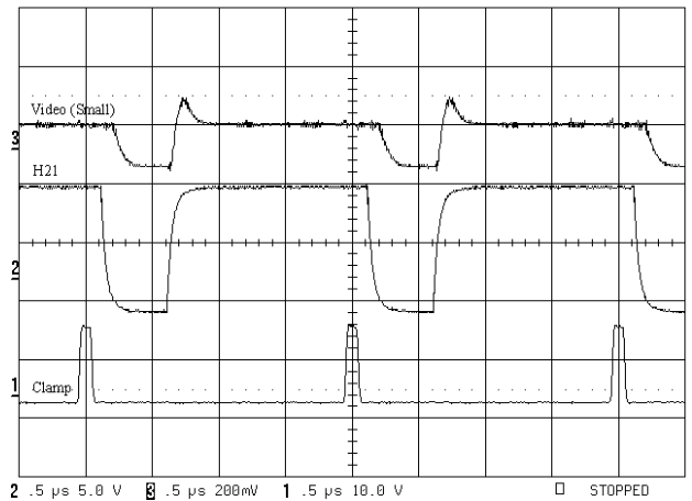
Figure 10 Two columns binned on to H21 (Video,H21,clamp clock)
