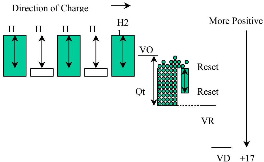
Figure 19 Charge lost over the Reset Gate
