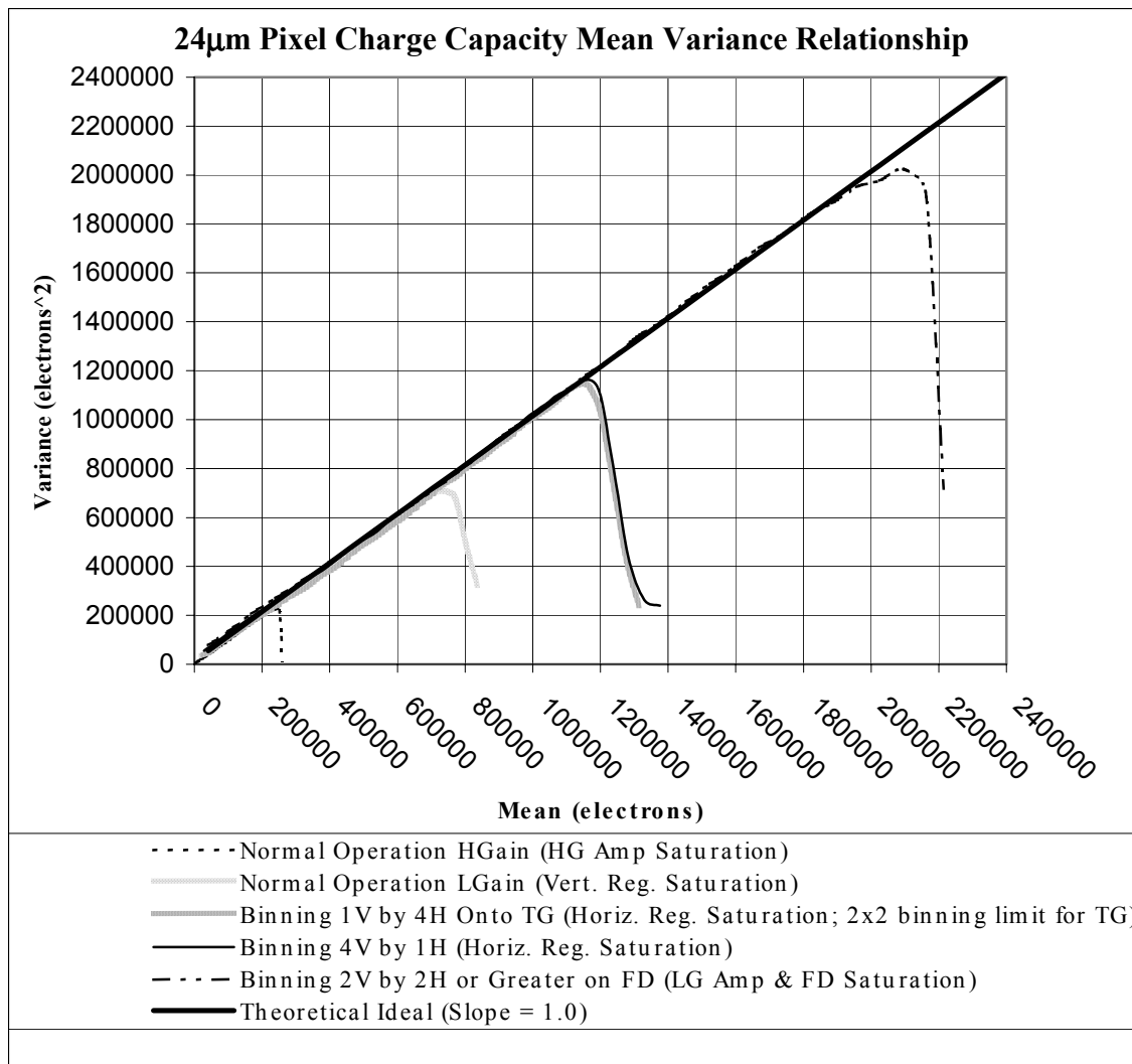
Figure 13 Mean-Variance Plot Showing Charge Capacities of Various Structures Using a Kodak 24μm Pixel Device in Various Modes
