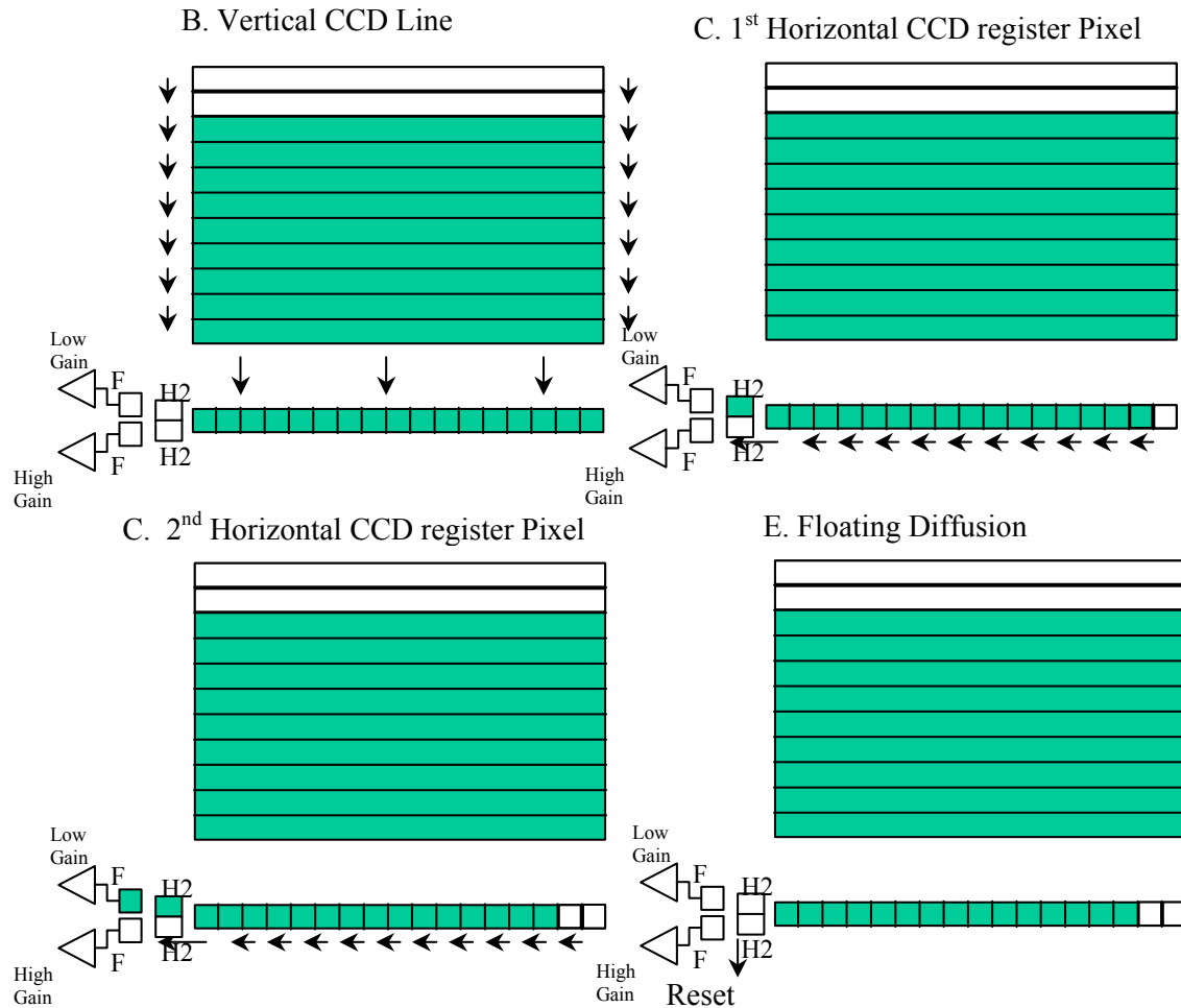
Figure 12 Charge Transport: 2X2 Binning On Transfer Gate (H21) Using Low Gain (2 \mu V/electron) Output
