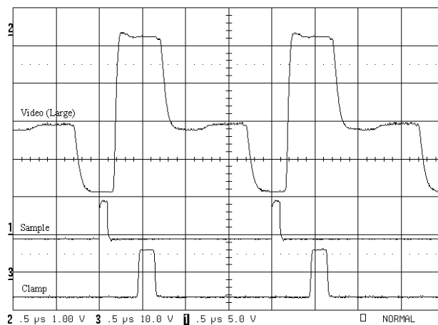
Figure 7 Two columns combined (binned) on to the floating diffusion (small signal)
