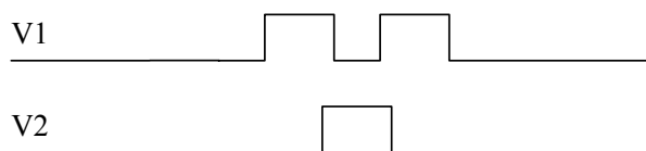
Figure 2 Normal vertical clock timing.
