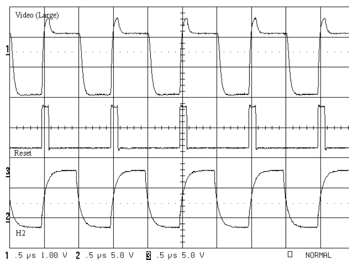
Figure 4 Normal pixel rate timing.
