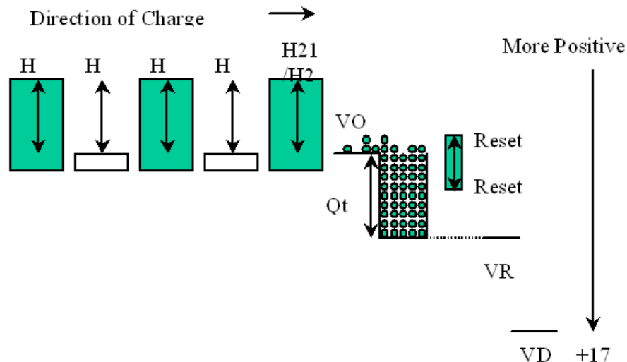
Figure 17 Charge Flowing back over VOG when the outthe floating diffusion capacity is reached.
