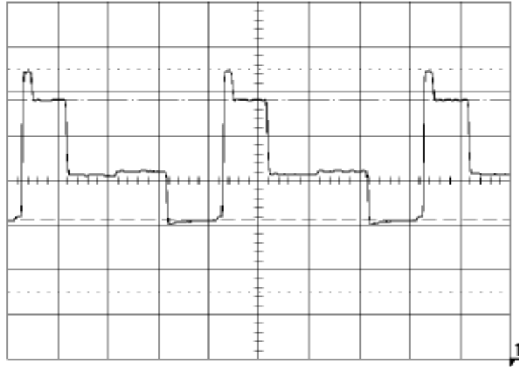
Figure 18 Charge lost over the Reset Gate
