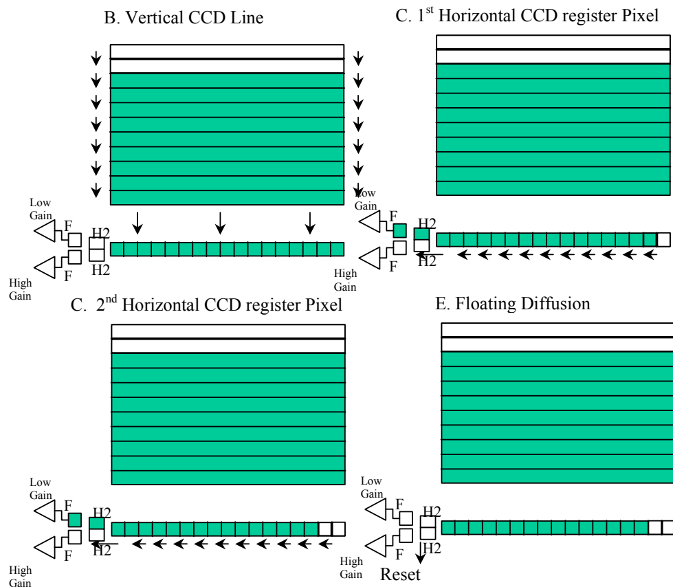
Figure 11 Charge Transport: 2X2 Binning On Floating Diffusion Using Low Gain (2μV/electron) Output
